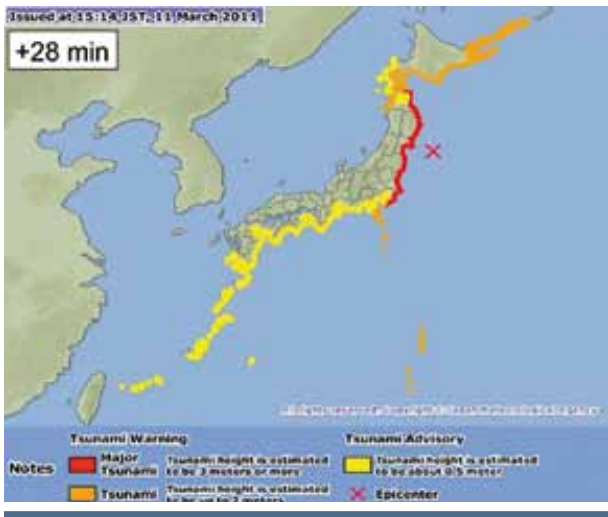
JMA tsunami forecast regions (left) and 11 March 2011 Japan tsunami warning (top). The entire eastern coast of Japan was placed on alert 28 minutes after the M9.0 earthquake, with northern Japan under a Major Tsunami and the rest of the Pacific coast under a tsunami warning or advisory. All warnings and advisories were cancelled after 2 days, 3 hours and 12 minutes.
